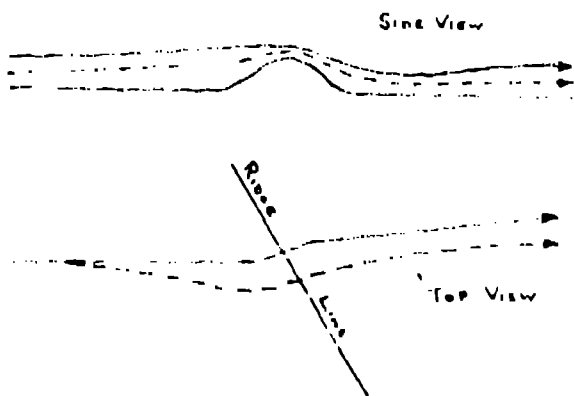
Fig. 3. Streamline deflections in vertical and horizontal views for flow over a simple ridge at 60° orientation to the mean flow.
