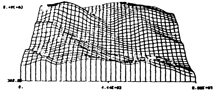
FIG. 4. An example of a computer-generated perspective view of the topography in the Cobble Mountain Anderson Creek Valley Area of northern California.
